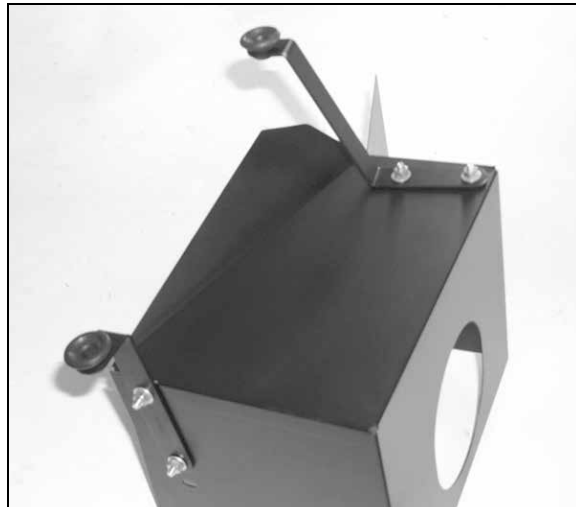
12. Install the "L" bracket onto the heat shield with the provided hardware. Do not tighten completely at this time.
