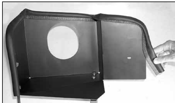
14. Install the provided edge trim onto the heat shield. Trim if necessary.
