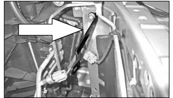
17a. On 2009 and later model vehicles, install the provided heat shield mounting bracket onto the radiator core support using the bolt removed in the previous step.
