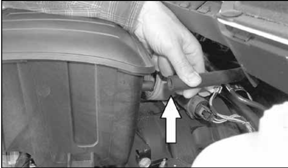
7. On 2002-2007 model year vehicles, disconnect the crank case vent hose from resonator box as shown. Then remove resonator box from vehicle. NOTE: K&N Engineering, Inc., recommends that customers do not discard factory air intake.
