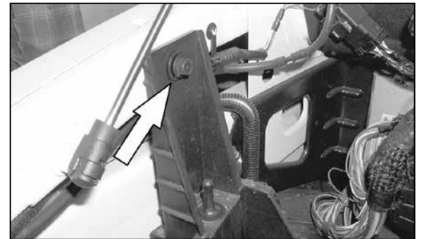
18. Remove the 8mm bolt that retains the air box mount.
