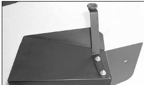
11. Install the large "Z" bracket onto the heat shield with the provided hardware. Do not tighten completely at this time.
