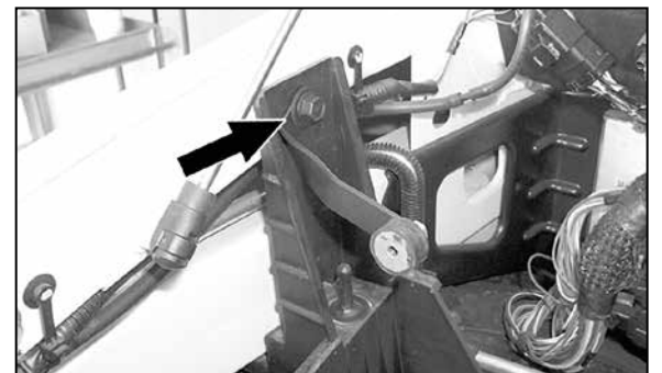
18a. Install the twisted "L" bracket with the bolt that was removed in step 18. Do not tighten bolt completely.
