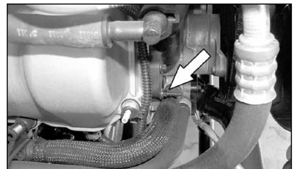
20. On 2002-2007 model year vehicles, use a 8mm socket, remove the stud that retains the oil fill bracket.
