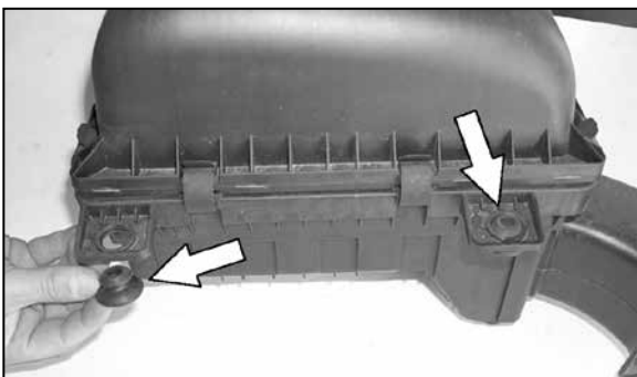
9. Remove the two rubber bushings from the factory air box as shown.
