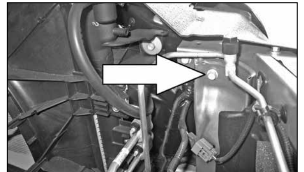
17. On 2009 and later model vehicles, remove the bolt shown from the radiator core support.
